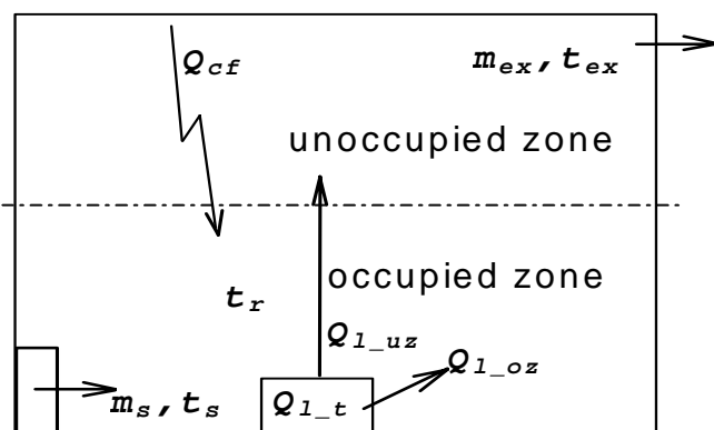
Figure 1 Room Energy Balance
