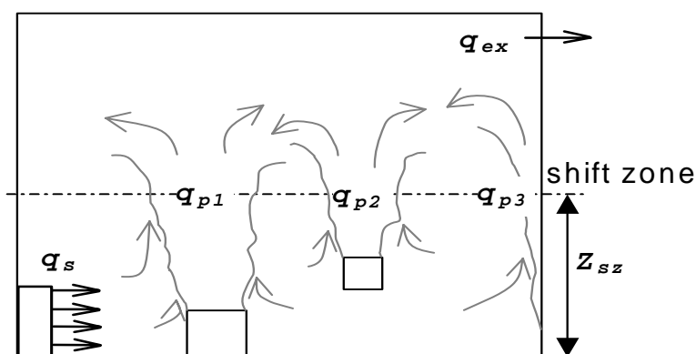
Figure 2 Shift Zone Design
