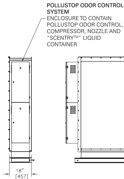
RIGHT HAND ACCESS SIDE ELEVATION
