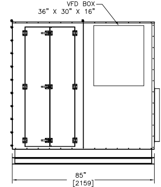
RIGHT HAND ACCESS SIDE ELEVATION
