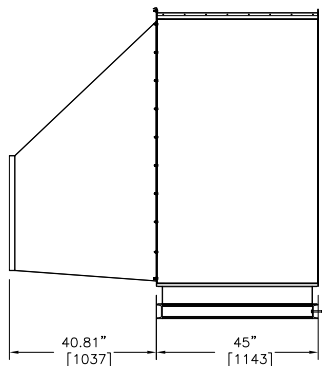
RIGHT HAND ACCESS SIDE ELEVATION
