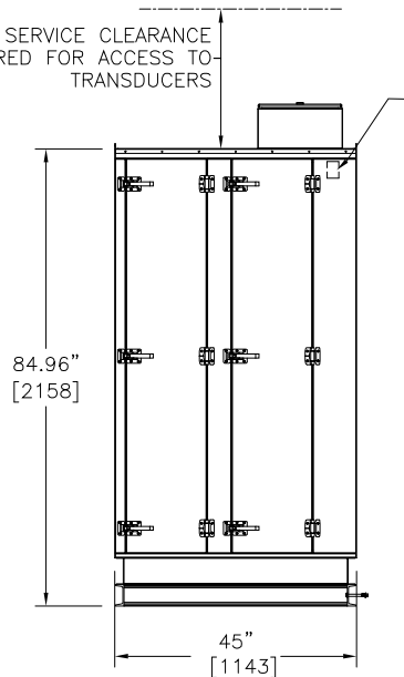
RIGHT HAND ACCESS SIDE ELEVATION
