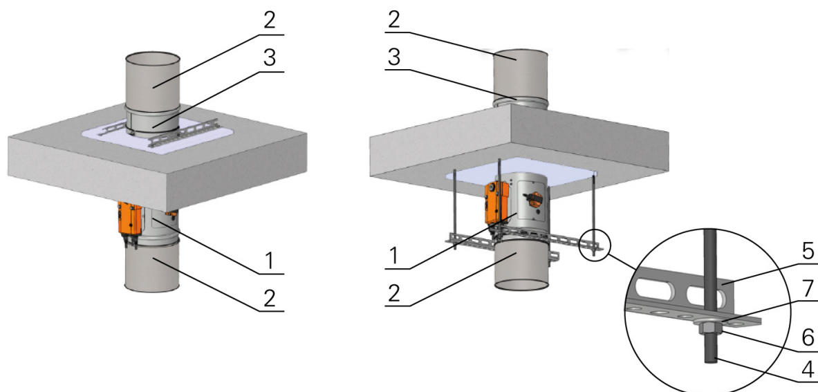
Fig. 12. Actuating mechanism below the floor construction
