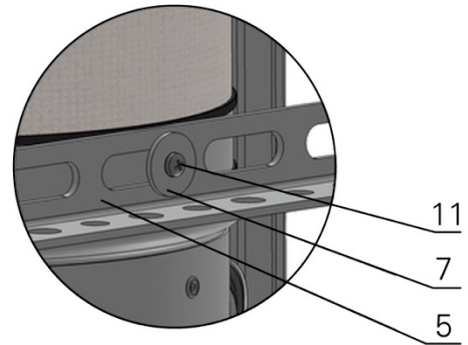
Fig. 14. Suspension ring and mounting rail connected by screw or rivet
