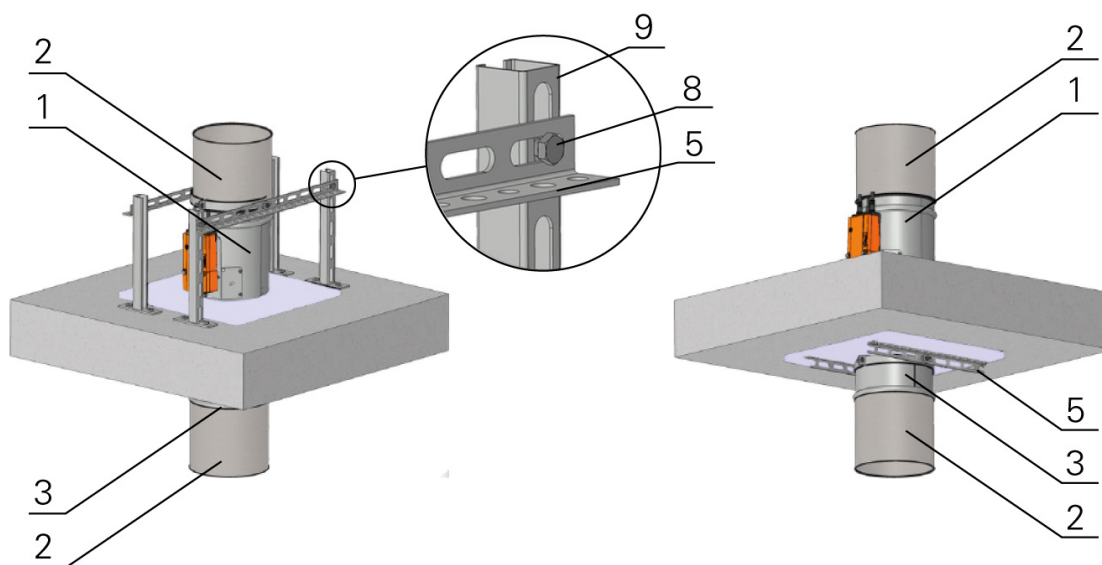
Fig. 11. Actuating mechanism above the floor construction
