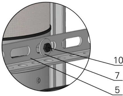
Fig. 13. Suspension ring and mounting rail connected by bolt
