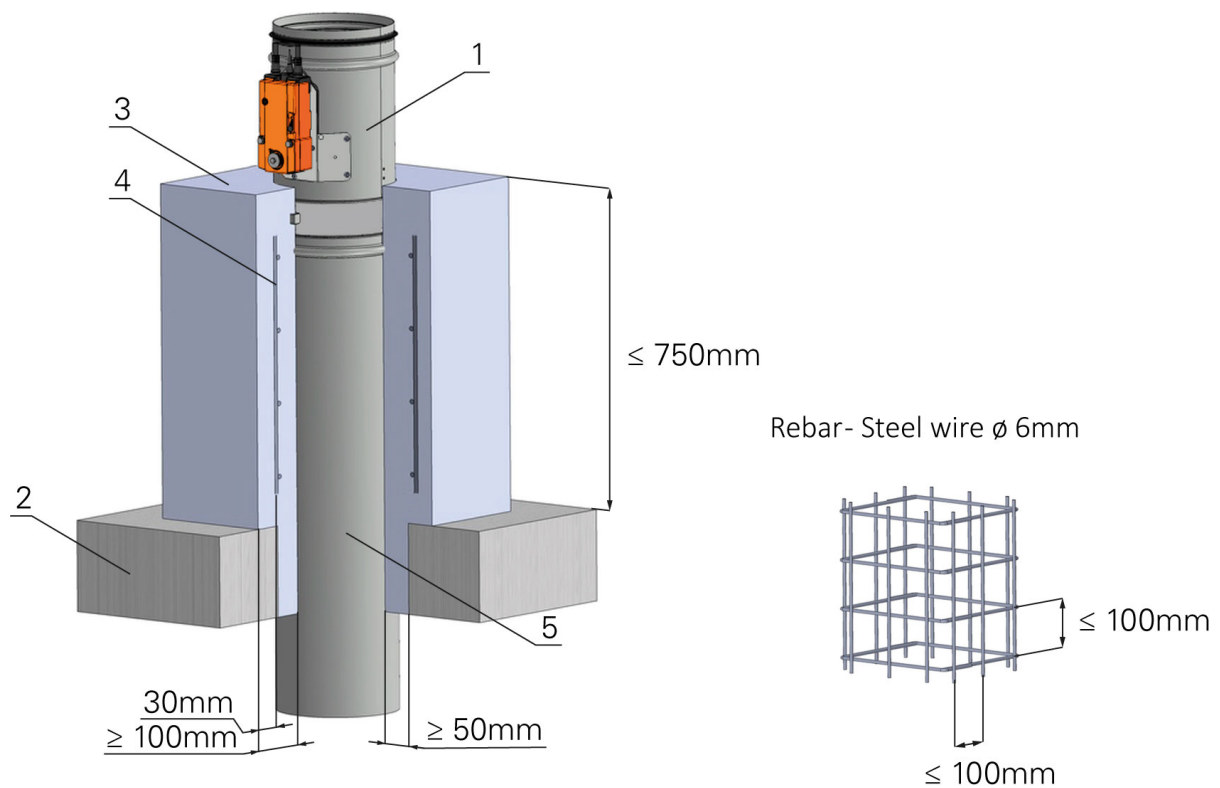
Fig. 9. Installation using concrete
