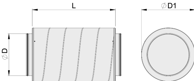
Fig. 1. Dimensions of circular sound attenuator
