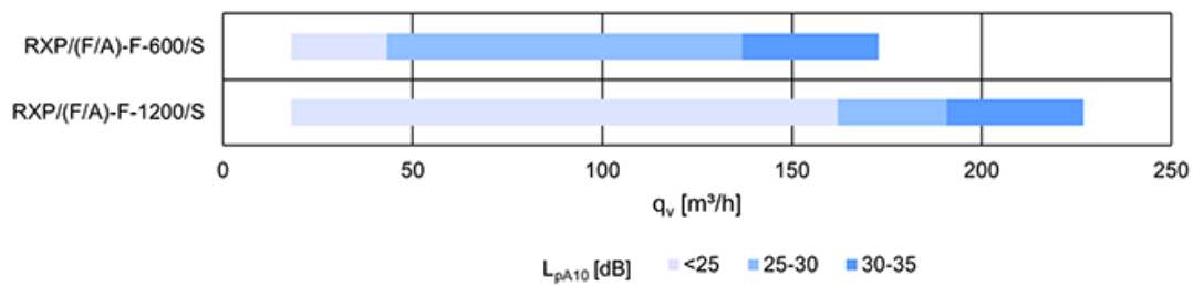
Fig. 17. Airflow ranges in m 3 /h for Halton Rex RXP, Flexible and Autonomic models @70 Pa total pressure
