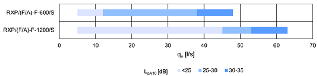
Fig. 16. Airflow ranges in l/s for Halton Rex RXP, Flexible and Autonomic models @70 Pa total pressure
