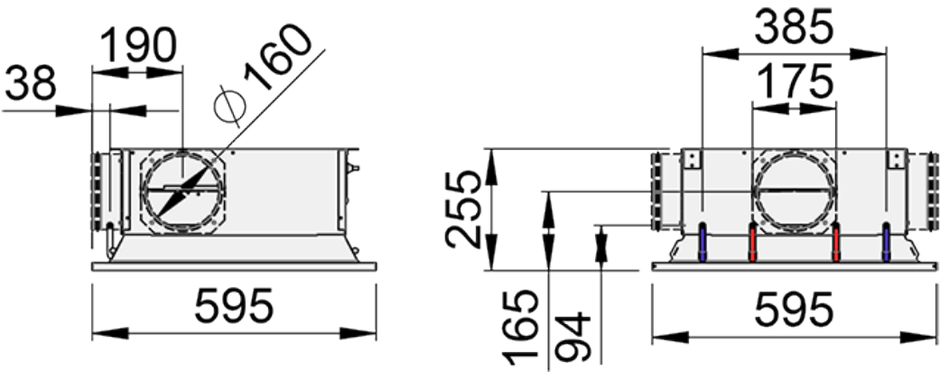
Fig. 22. Halton Rex RXP, Flexible and Autonomic models dimensions (RXP/F-600 or RXP/A-600)
