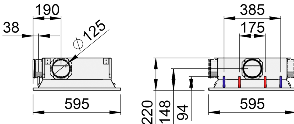
Fig. 19. Halton Rex RXP, Standard model dimensions (RXP/S-600)
