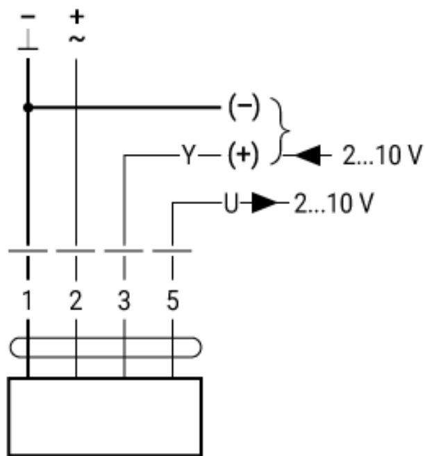
Fig. 34. Connection diagram analog for Halton Rex RXP, Autonomic model
