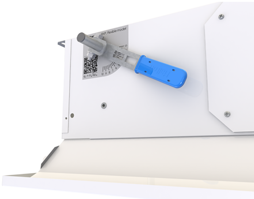
Fig. 27. Adjustment of the manual actuator position in Halton Rex RXP, Flexible model
