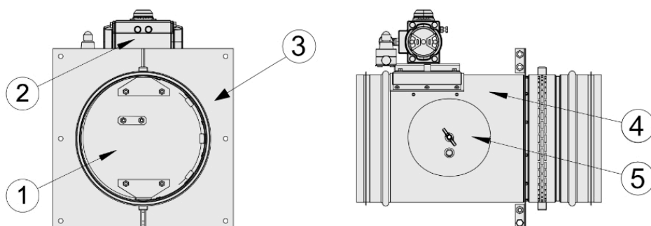
Fig. 1. Halton Ivo ITC structure
