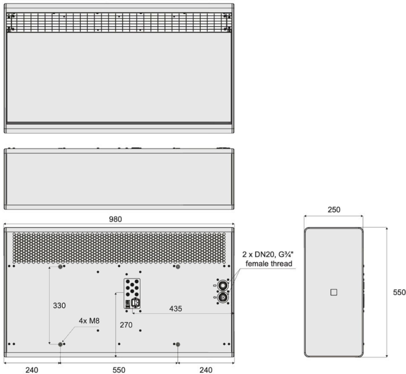
Fig. 3. Dimensions of Halton Windis DWE
