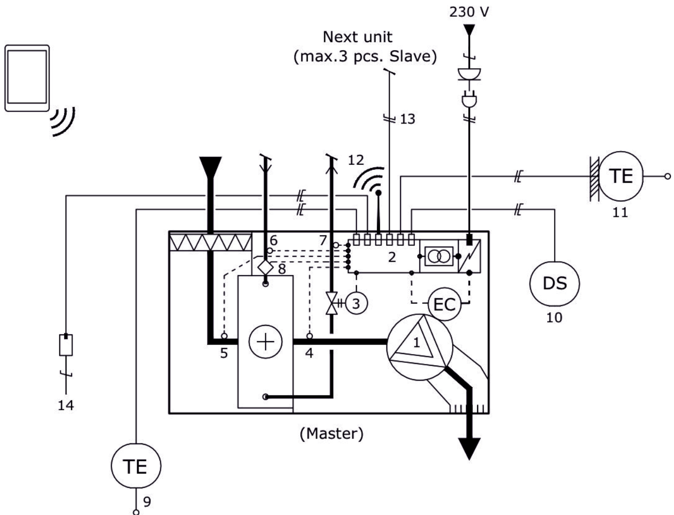
Fig. 4. Halton Windis DWE connection diagram
