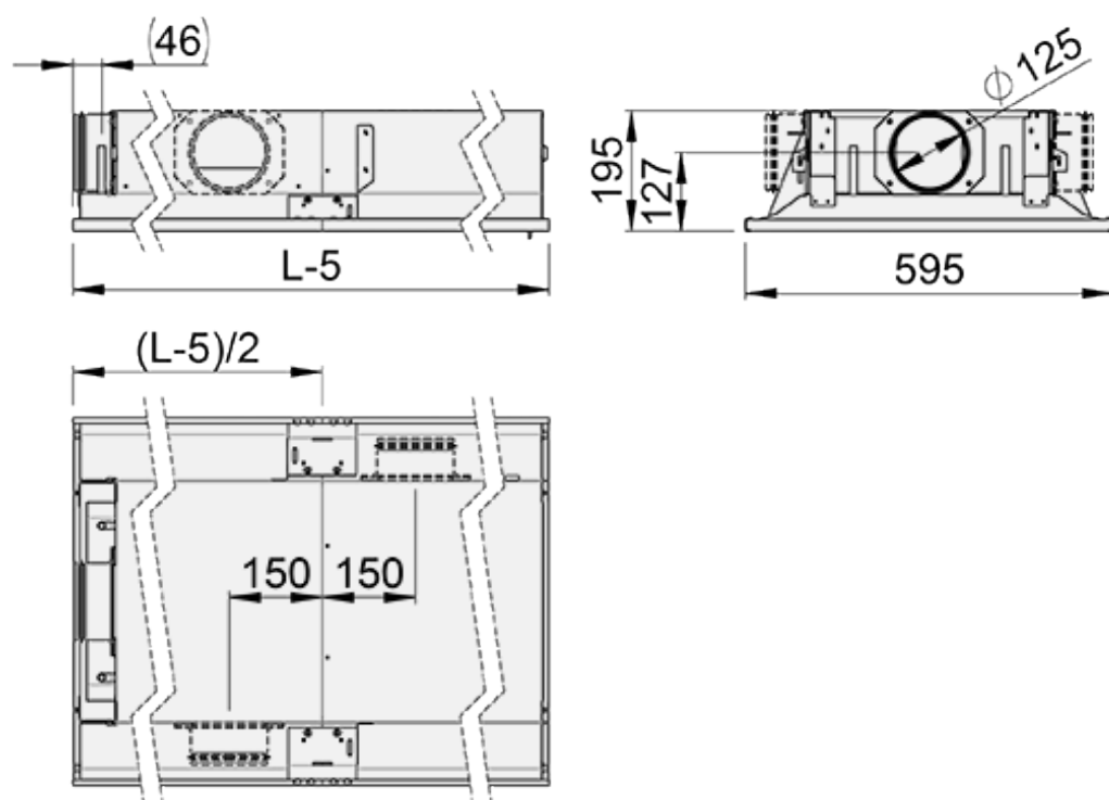
Fig. 6. Total length 2500 – 3600 mm
