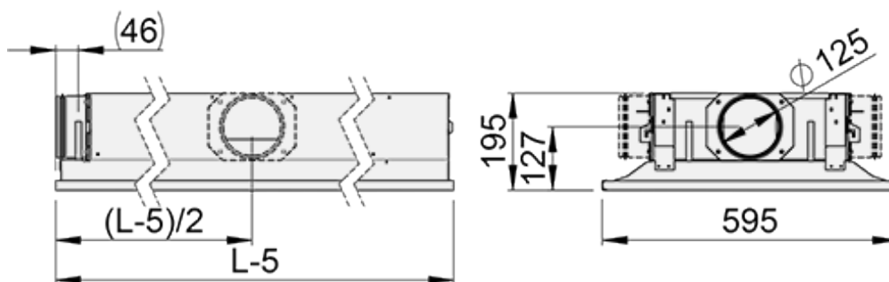
Fig. 5. Total length 1200 - 2400 mm
