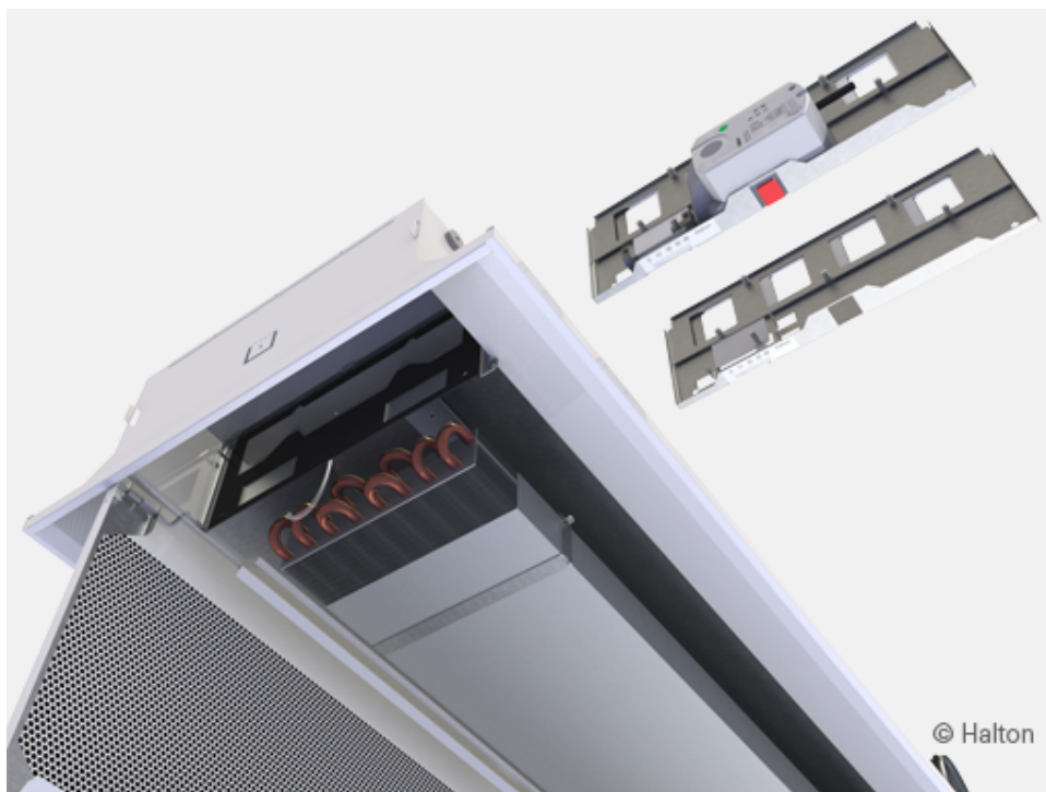
Fig. 22. Halton Rex RE6, HAQ replacement
