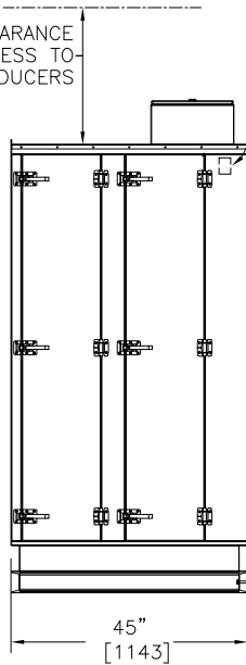
RIGHT HAND ACCESS SIDE ELEVATION
