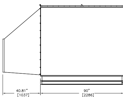
RIGHT HAND ACCESS SIDE ELEVATION
