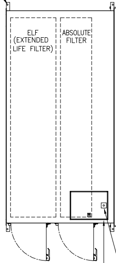
PLAN VIEW
