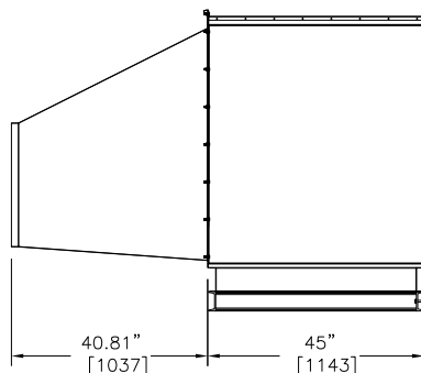
RIGHT HAND ACCESS SIDE ELEVATION
