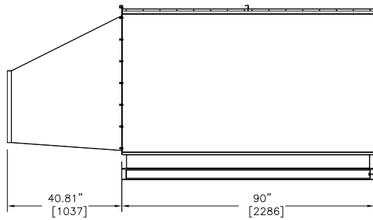
RIGHT HAND ACCESS SIDE ELEVATION
