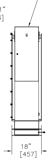
RIGHT HAND ACCESS SIDE ELEVATION
