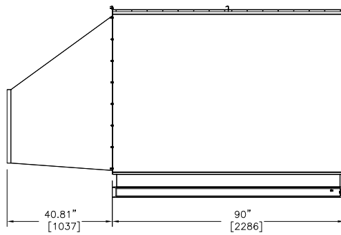
RIGHT HAND ACCESS SIDE ELEVATION
