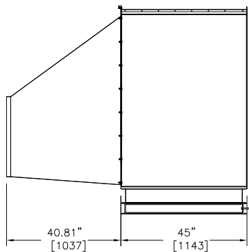
RIGHT HAND ACCESS SIDE ELEVATION
