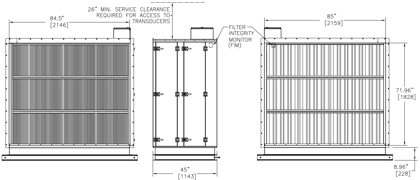
LEFT END VIEW
