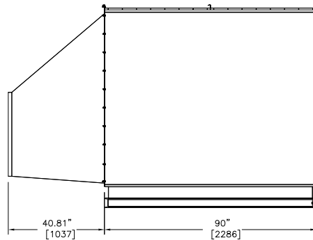
RIGHT HAND ACCESS SIDE ELEVATION
