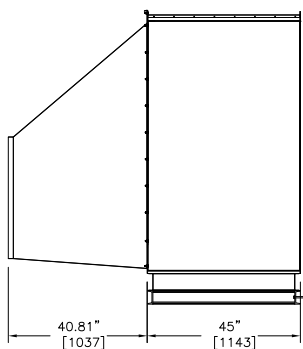
RIGHT HAND ACCESS SIDE ELEVATION
