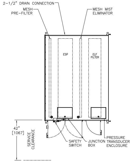
PLAN VIEW
