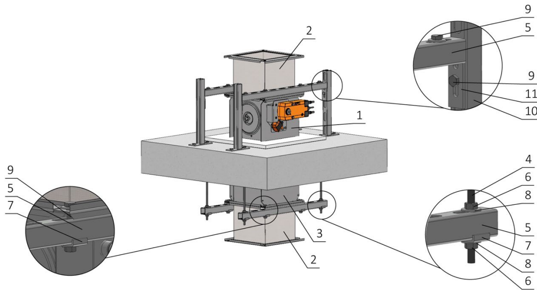
Fig. 12. Actuating mechanism above the floor construction
