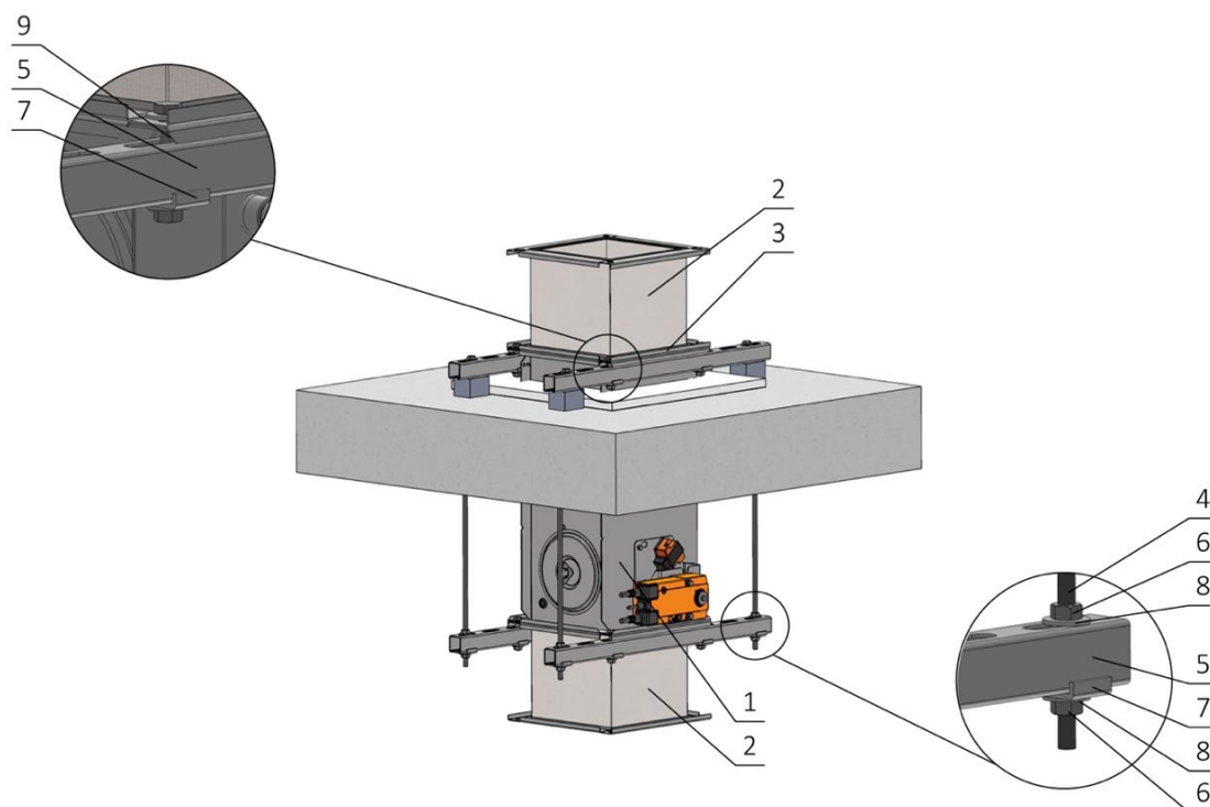
Fig. 13. Actuating mechanism below the floor construction
