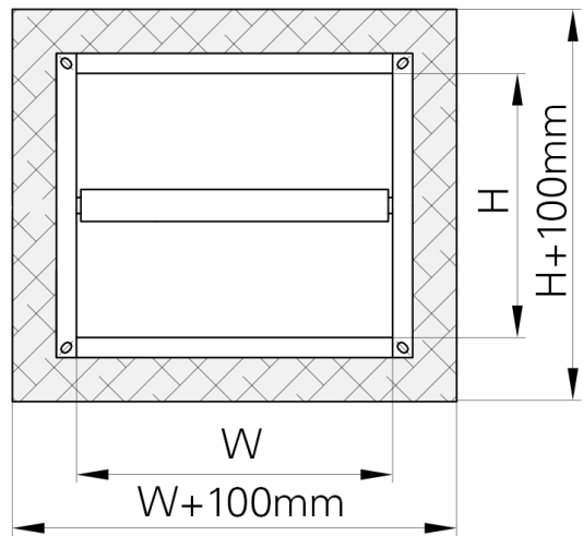
Fig. 2. Installation opening, rectangular
