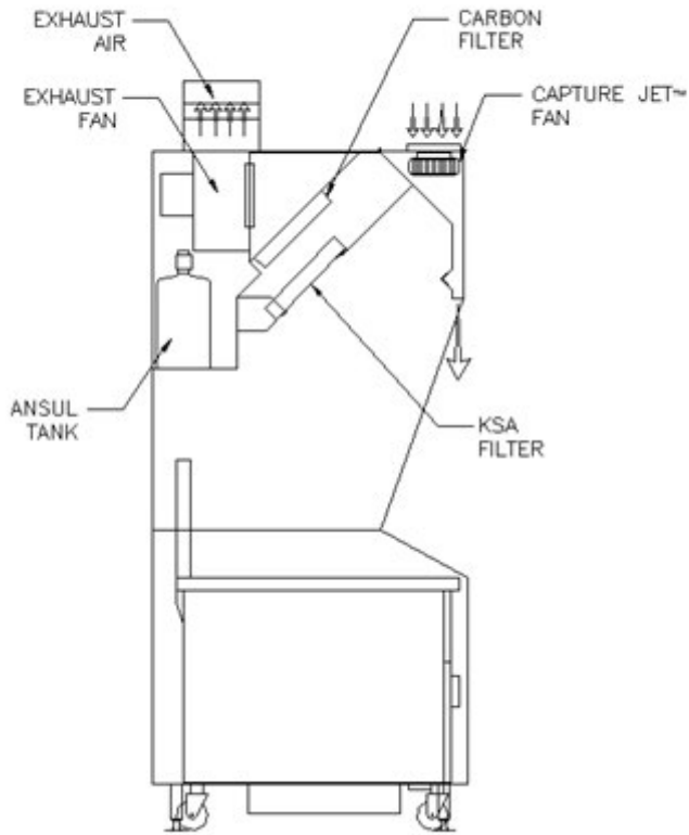
LIFT FILTER INTO PLENUM
