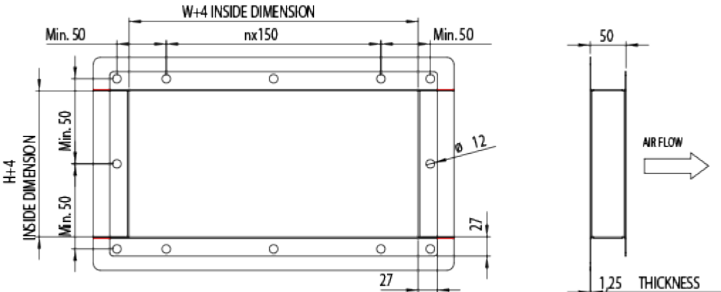
*Drilling pattern according to Eurovent
