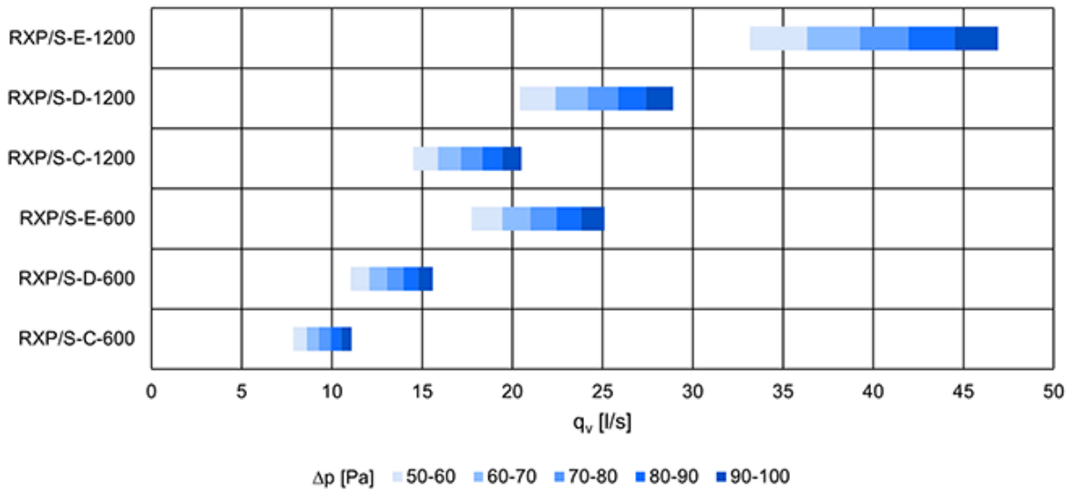
Fig.14. Airflow ranges in l/s for Halton Rex RXP, standard model without HAQ/with HAQ closed with different static chamber pressure levels
