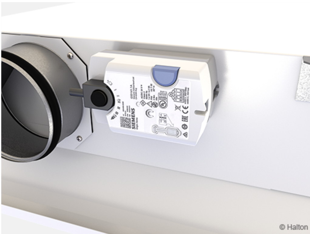
Fig.5. Electric actuator of HAQ control in Halton Rex RXP, Standard model
