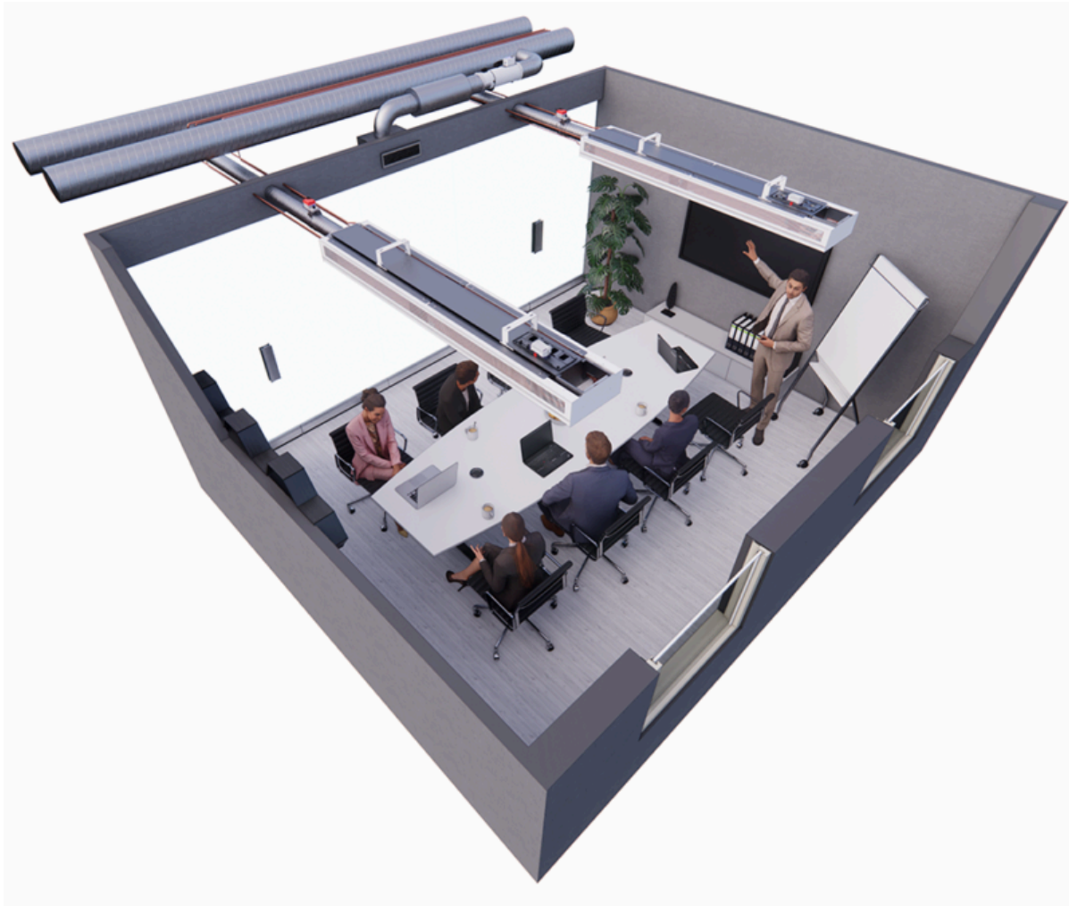
Fig. 12: Halton Rex Exposed (REE) active chilled beams with HAQ control and PTS damper, controlled with Halton Workplace WRA room automation controllers in a meeting room
