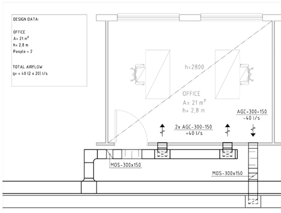
Fig. 8. Halton Max MOS ventilation design
