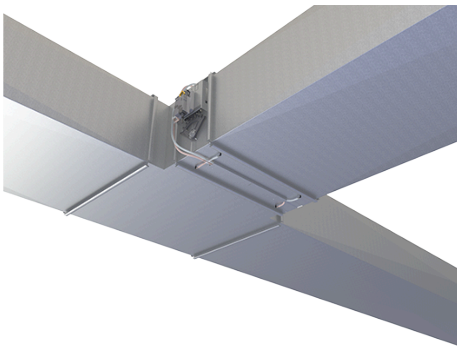
Fig. 5. Example of Halton Max MOS installed to duct with no safety distances
